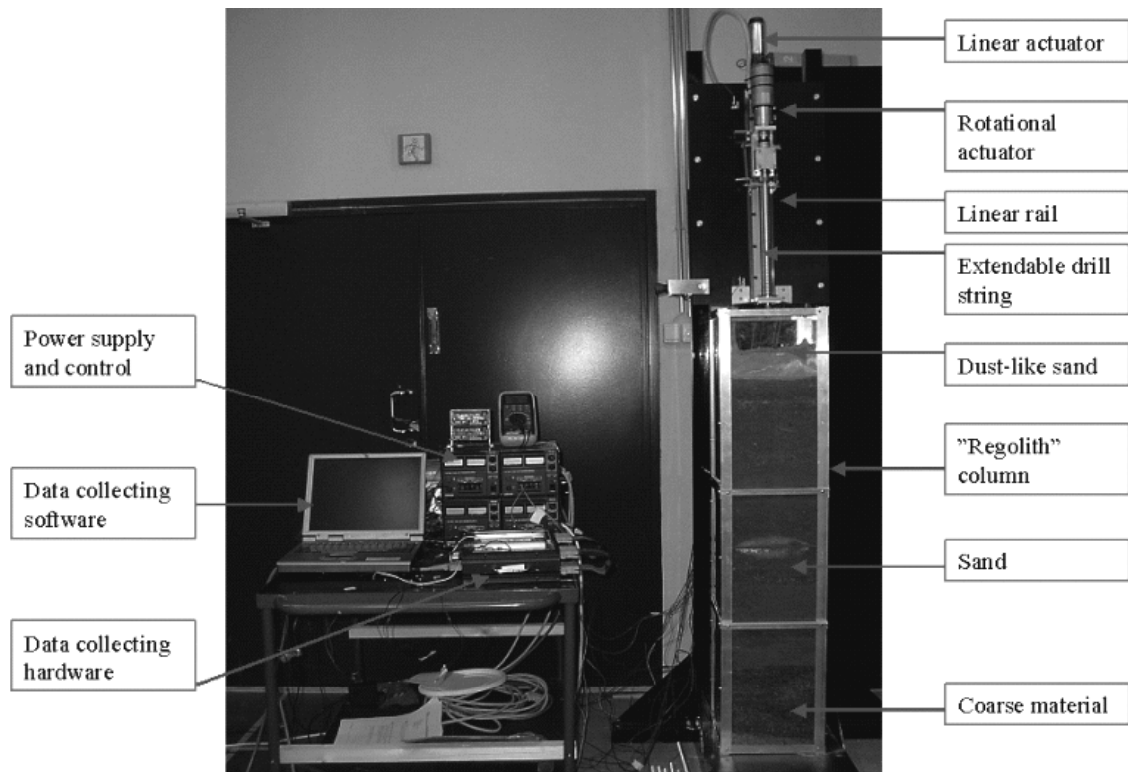
Fig. 2: The principle of the MIRANDA drilling test bench (Image: MA).
