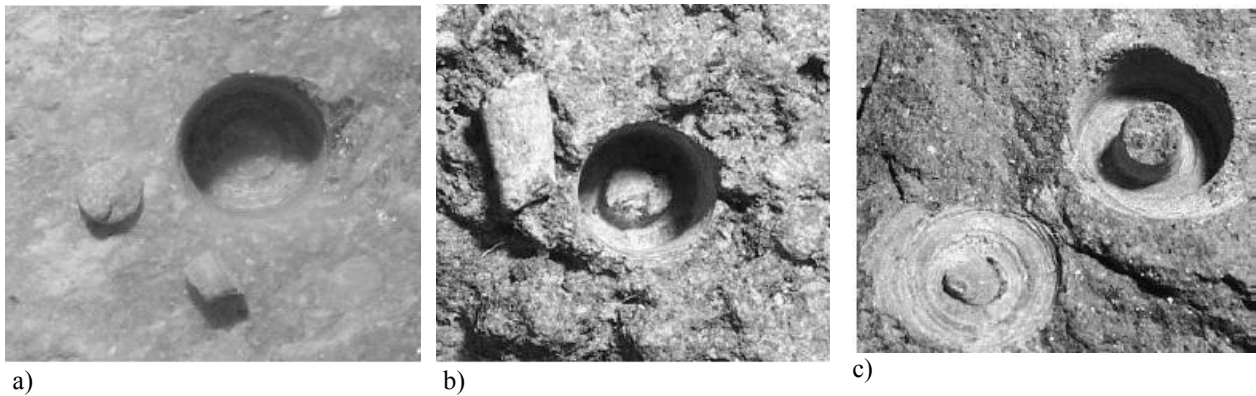
Fig. 3: Carbonatite (a) and diabase (b) drilling holes and the corresponding retrieved core pieces. The borehole is 17 mm in diameter. Mafurite is shown in c) and the core sample has not yet been extracted (Images: MA).
