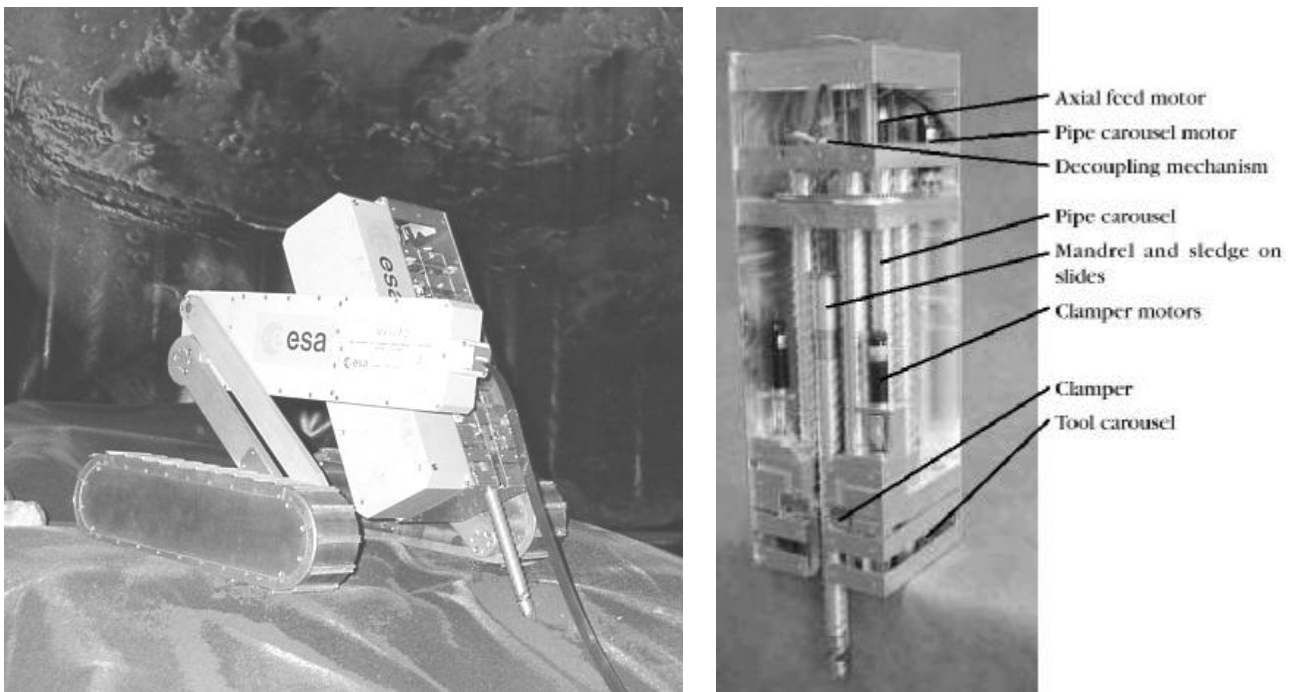
Fig. 1: The MRoSA2 rover in drilling position (Image: SSF). The DSS module is shown on the right (Image: VTT).
